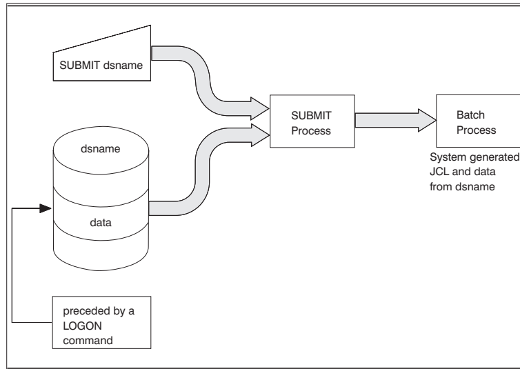
Figure 6. The SUBMIT Process Using System-Generated JCL
