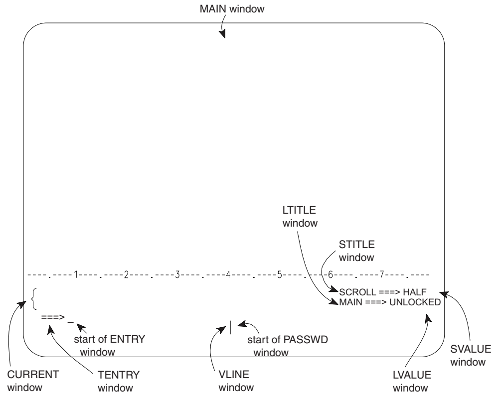
Figure 12. Session Manager Display Screen
