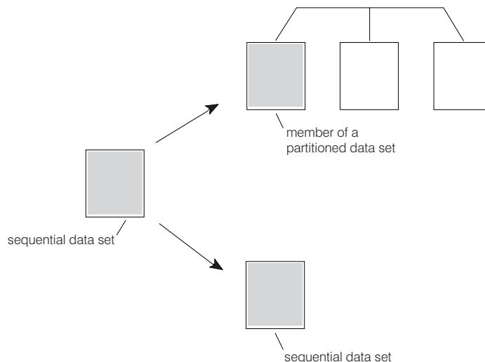
Figure 3. Copying a Sequential Data Set
